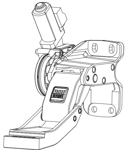
③ x2 Motor Linkage
