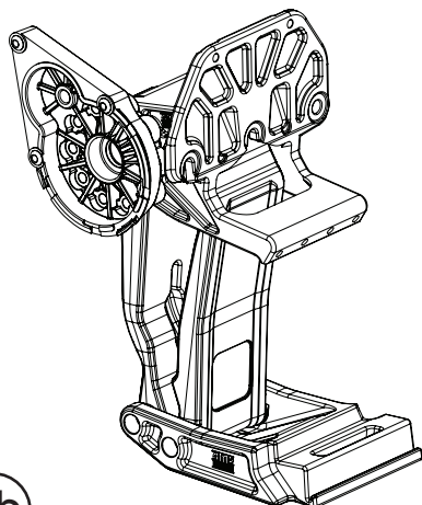
Rear Motor Linkage Assembly - Passenger Side
